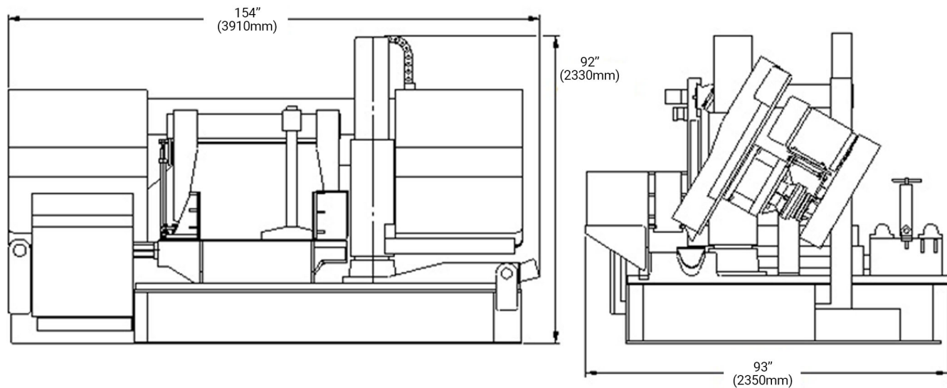
Dimensional Drawings of DC-700NC
