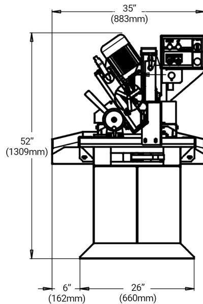
Dimensional Drawings of DS-280M
