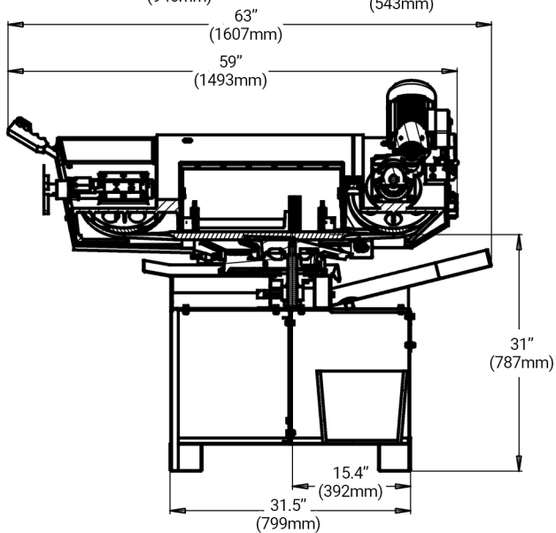
Dimensional Drawings of DS-280M
